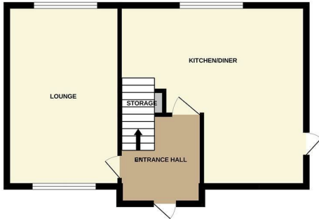
GROUND FLOOR 456 sq.ft. (42.4 sq.m.) approx.
